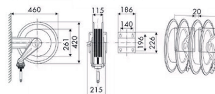
OVERALL DIMENSIONS (mm)
